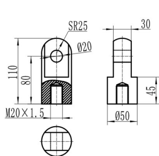
叉销端GA
